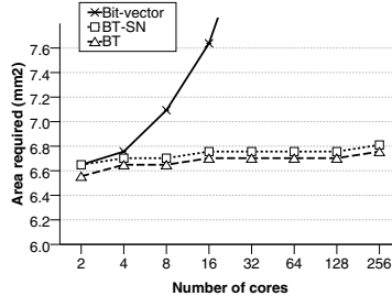
Fig. 3. Area ( \text{mm}^2 ) required for a 1MB cache module when bit-vector, BT or BT-SN are used
