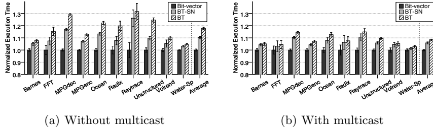
Fig. 5. Execution time for 32 cores
