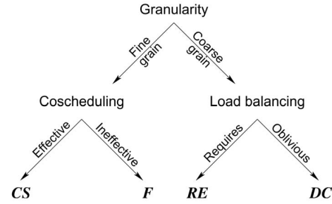
Fig. 1. Decision tree for process classification.
