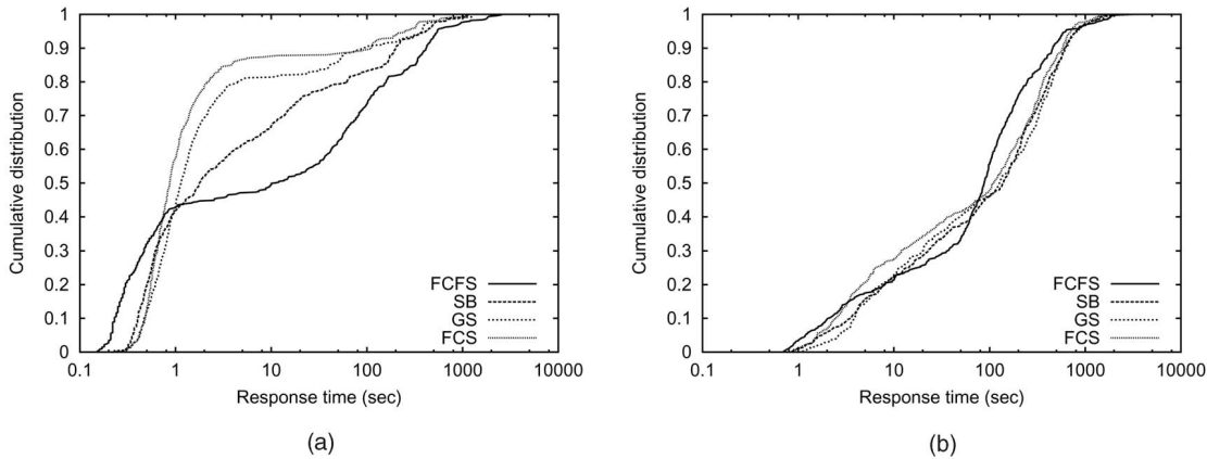
Fig. 8. Cumulative distribution of response times at 74 percent load and FCS scheduling. (a) 500 shortest jobs. (b) 500 longest jobs.
