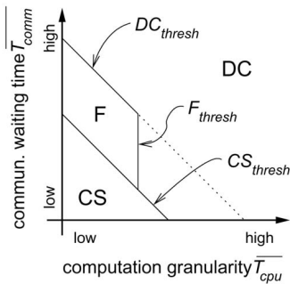
Fig. 2. Phase diagram of classification algorithm.
