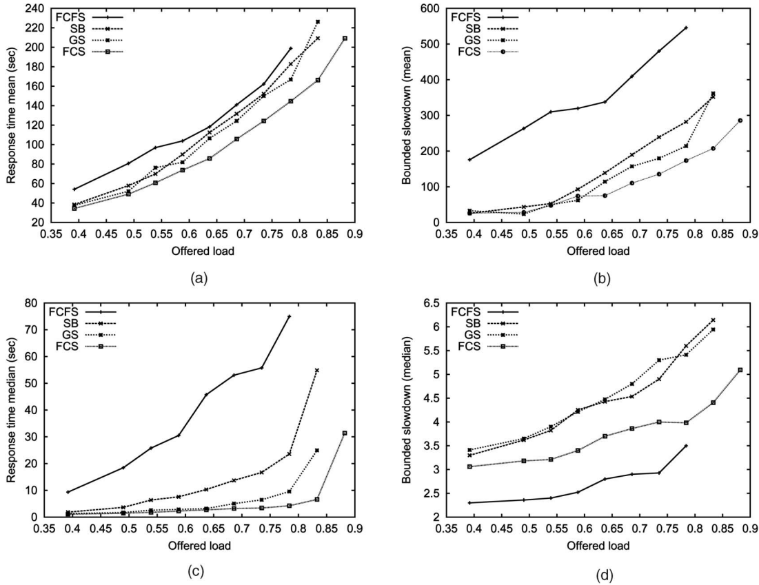
Fig. 7. Performance as a function of offered load—synthetic applications. (a) Mean response time. (b) Mean bounded slowdown. (c) Median response time. (d) Median bounded slowdown.
