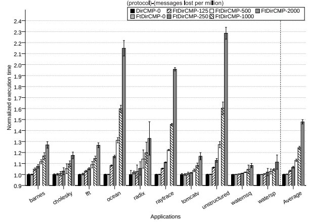
Figure 3. Execution time overhead of FTDIRCMP compared to DIRCMP for several fault rates.
